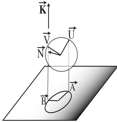
Figure 11: The coin is projected onto an ellipse in the camera plane.
