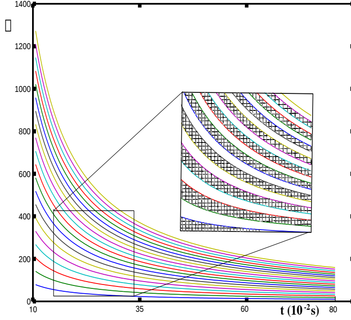
Figure 6: The hyperbolas separating heads from tails in part of phase space. Initial conditions leading to heads are hatched, tails are left white, \omega is measured in s^{-1} .
