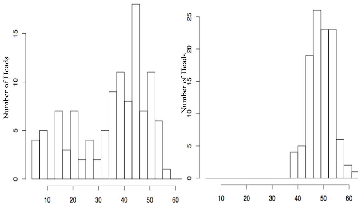
Figure 7a: Coins spun on their edges
