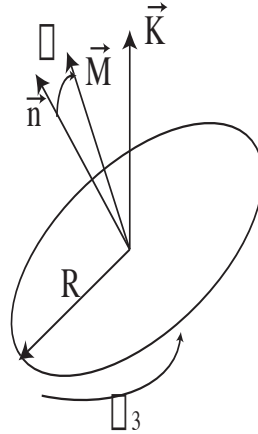
Figure 2b: Coordinates of Precessing Coin, \vec{K} is the upward direction, \vec{n} is the normal to the coin, \vec{M} is the angular momentum vector, \omega_3 is the rate of rotation around the normal \vec{n} .
