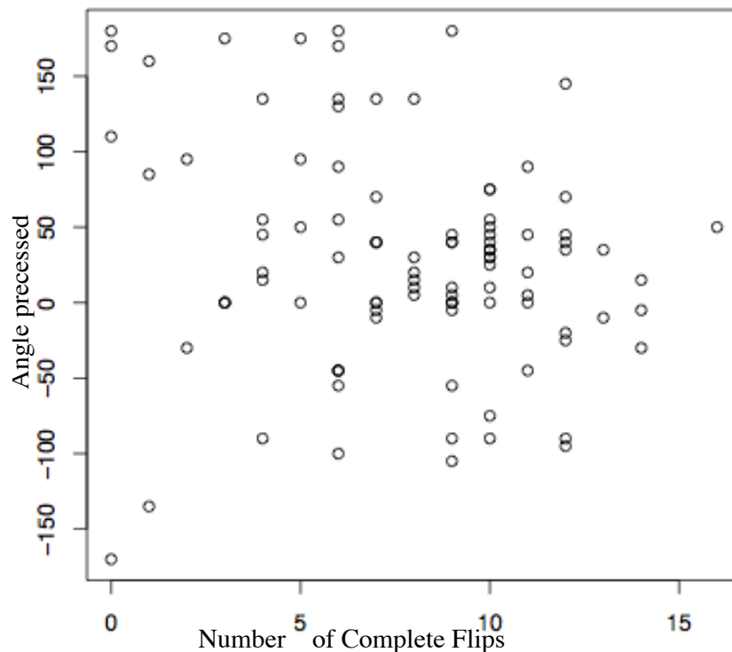
Figure 10: Scatterplot of ribbon data
