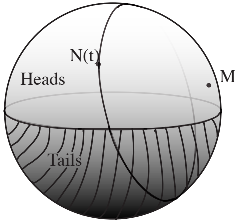
Figure 4: The normals to the coin lie on a circle intersecting with the equator of change of sides from Heads to Tails (hatched area).
