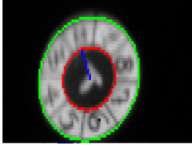
Figure 12: Fit of two ellipses to the image.
