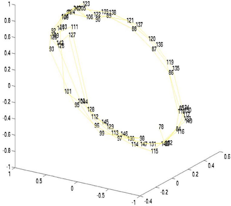
Figure 13b: How the normal vectors (once unscrambled) sit around a circle in 3-D.
