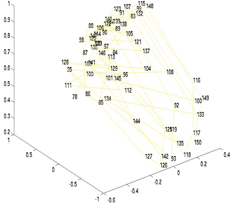
Figure 13a: The normals originally have a scrambled sign pattern.
