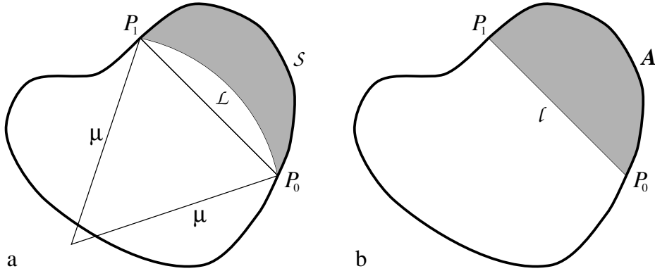
Figure 3: When T is a twist map, its generating function G can be expressed (a) as a function of the length \mathcal{L} of \gamma and the area \mathcal{S} between \gamma and \partial Q , or (b) as a function of the length \ell of P_0P_1 and the area A between P_0P_1 and \partial Q .
