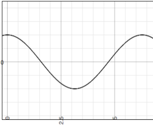
FIGURE 1. The graph of \cos(x) .
