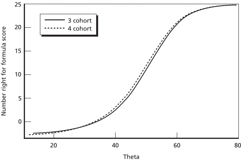
Figure A.1 Test Characteristic Curve, All 25 Mathematics Items
