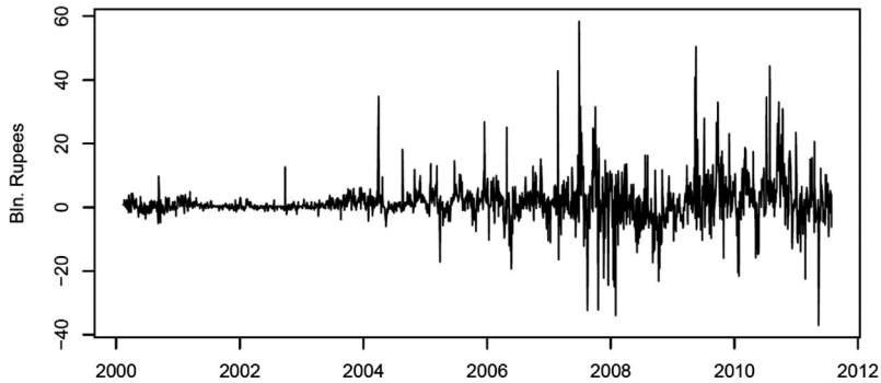
Figure 1: Net FII Flows
