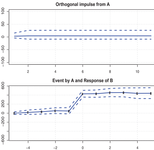
Figure 3: Monte Carlo experiment
