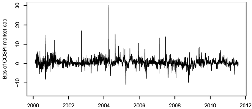
Figure 2: Normalized Net FII Flows
