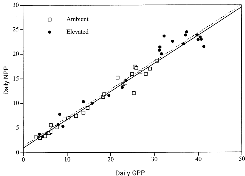
Fig. 7 Linear correlation between daily NPP and daily GPP under ambient CO 2 and elevated CO 2 .
