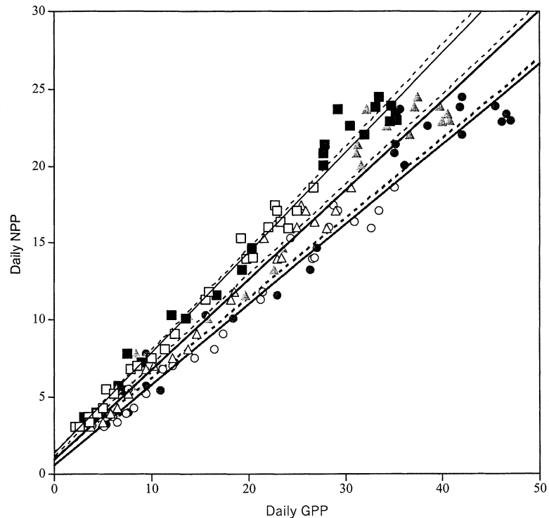
Fig. 8 Linear correlation between daily NPP and daily GPP under ambient CO 2 and elevated CO 2 when three different Q_{10} values are used to calculate daytime shoot respiration. Open symbols are data points of the ambient CO 2 treatment. Closed symbols are data points of the elevated CO 2 treatment. Square symbols are data points when Q_{10}=1.5 , triangle symbols are data points when Q_{10}=2.0 , and circle symbols are data points when Q_{10}=2.5 . Dotted lines are linear fits of data points of the ambient CO 2 treatment, and solid lines are linear fits of data points of the elevated CO 2 treatment. The middle two lines are linear fits of data points when Q_{10}=2.0 , which are the same as shown in Fig. 7. The upper two lines are linear fits of data points when Q_{10}=1.5 , and the lower two lines are linear fits of data points when Q_{10}=2.5 .
