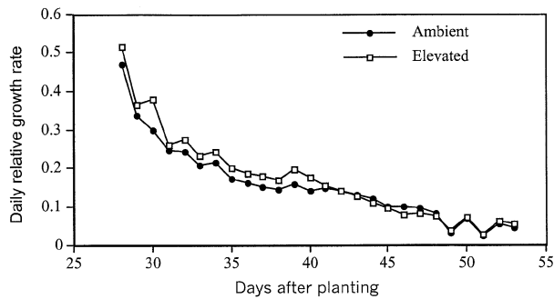
Fig. 4 Daily relative growth rates ( \text{g C g C}^{-1} \text{d}^{-1} ) under ambient \text{CO}_2 and elevated \text{CO}_2 .
