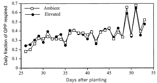
Fig. 5 Daily fraction of GPP respired by the plants under ambient \text{CO}_2 and elevated \text{CO}_2 .
