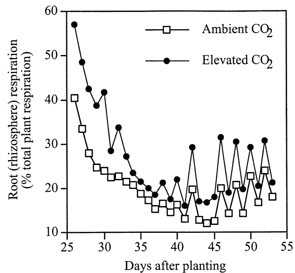
Fig. 6 Root/rhizosphere respiration as percentage of total daily plant respiration under ambient \text{CO}_2 ( \square ) and elevated \text{CO}_2 ( \bullet ).
