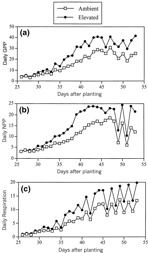
Fig. 1 (a) Daily gross primary production (GPP), (b) daily net primary production (NPP), and (c) daily total plant respiration (respiration) in \text{gC m}^{-2} \text{d}^{-1} .
