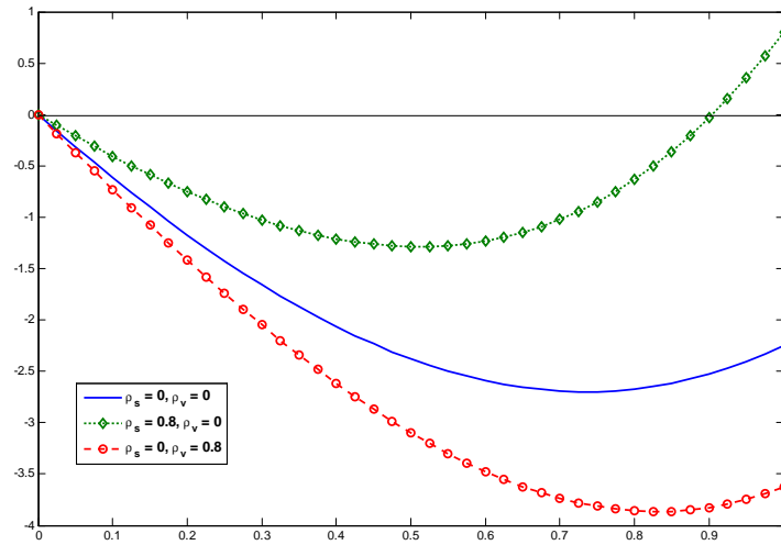
Figure 1: Effects of transparency on loss (percent change relative to P = 0 )
