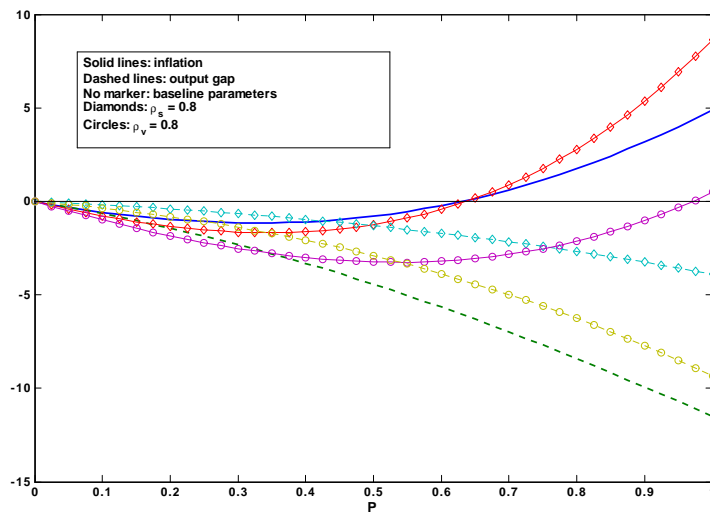
Figure 2: Effects of transparency on variances (percent change relative to P = 0 )
