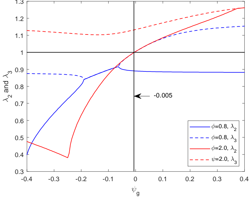
Figure A1: Eigenvalues \lambda_2 and \lambda_3 as a function of \psi_g for \phi = 0.8 (blue) and \phi = 2.0 (red). The vertical line is at \psi_g = -\rho = -0.005 .
