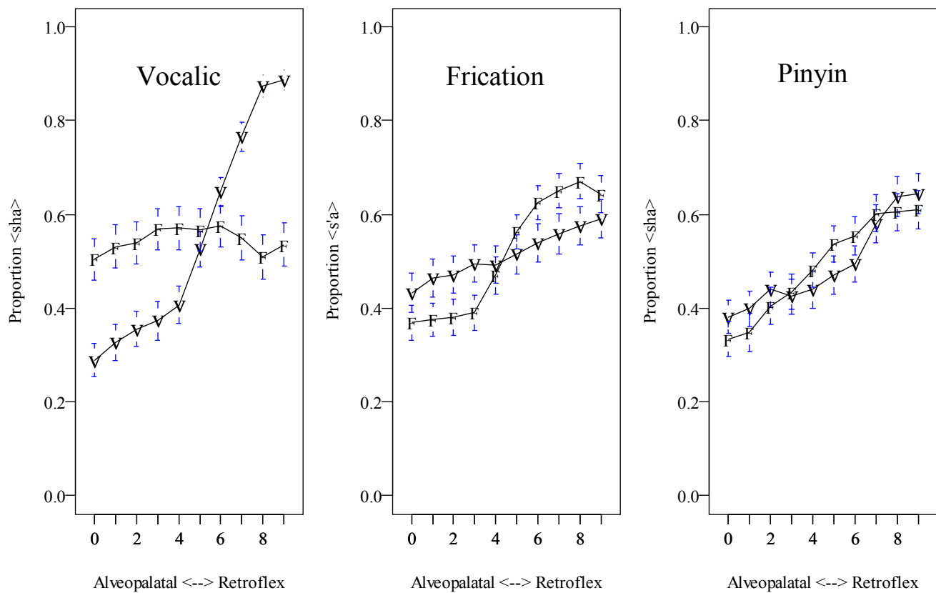
Fig. 1. Proportion \langle sha \rangle / \langle s'a \rangle responses for each group. F = frication dimension, V = vocalic dimension. Leftmost panel represents the vocalic group, middle panel the frication group, rightmost panel the pinyin group.
