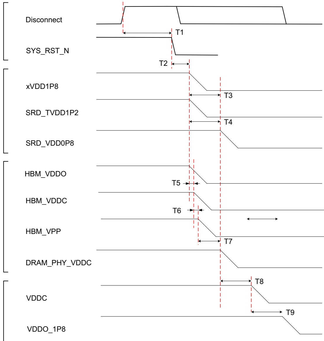
Figure 11: Power-Down Sequence
