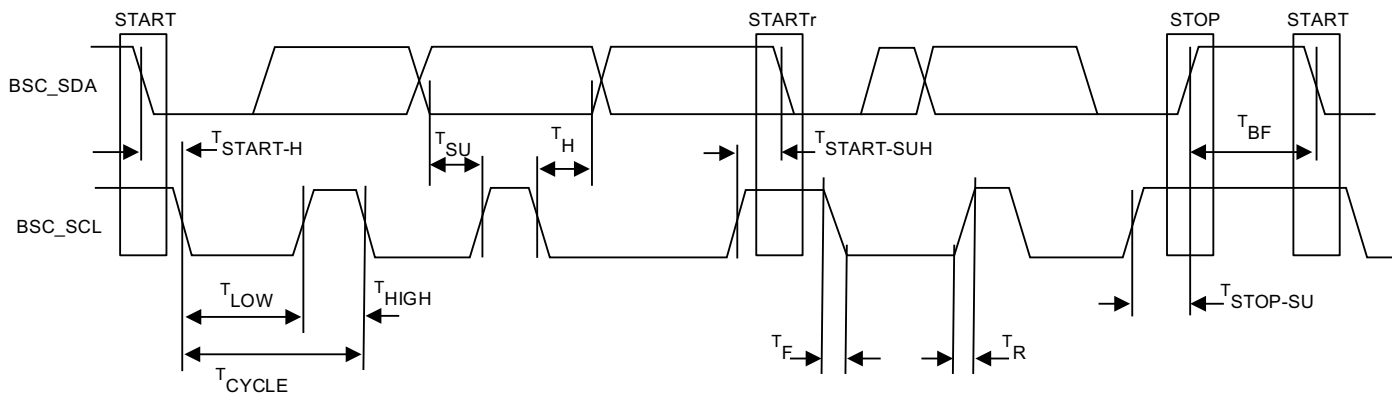
Figure 14: BSC Timing Diagram
