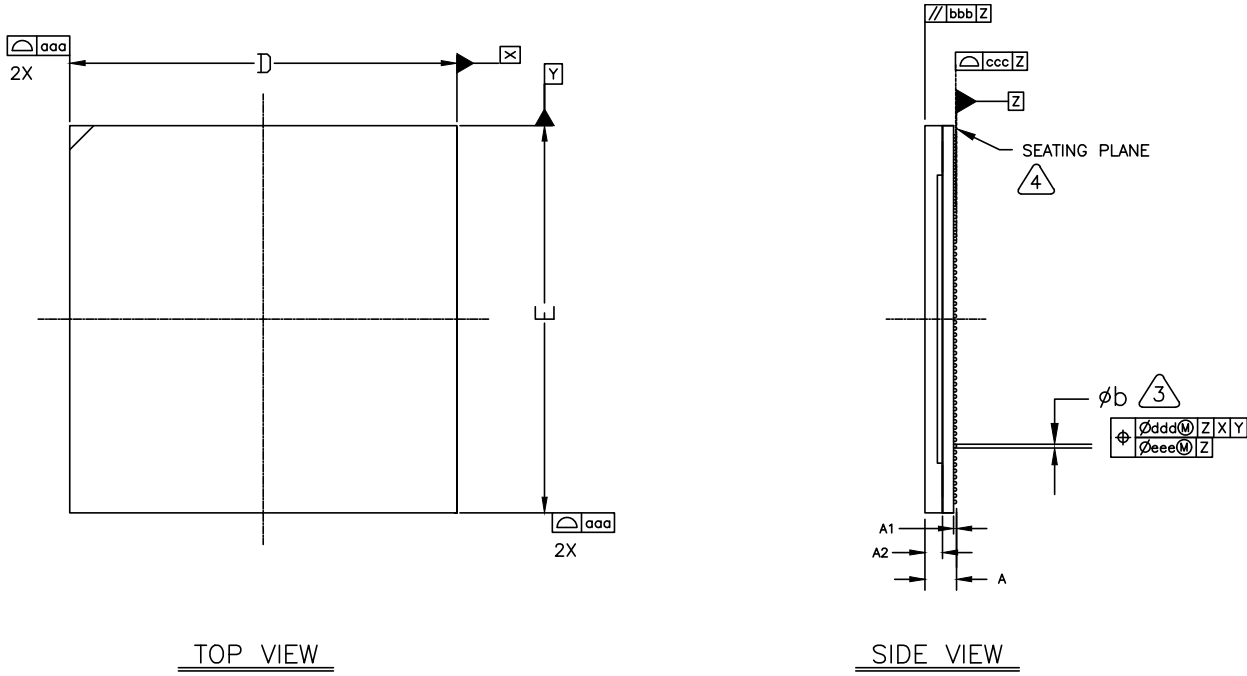
Figure 25: Package Outline
