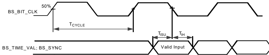
Figure 20: BroadSync Input Timing – Slave Mode
