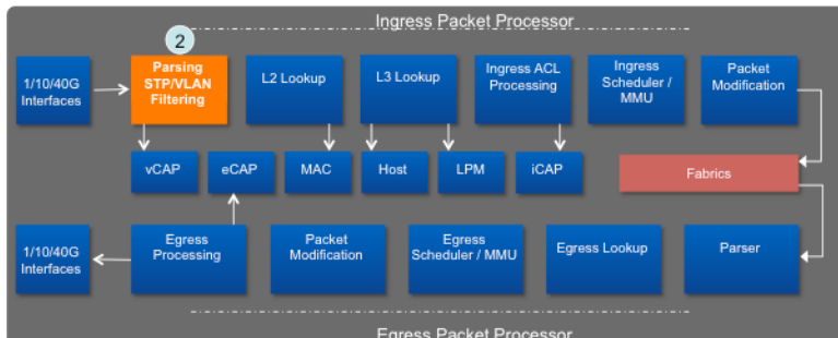
Figure 14: Packet Processor stage 2: Ingress Parser
