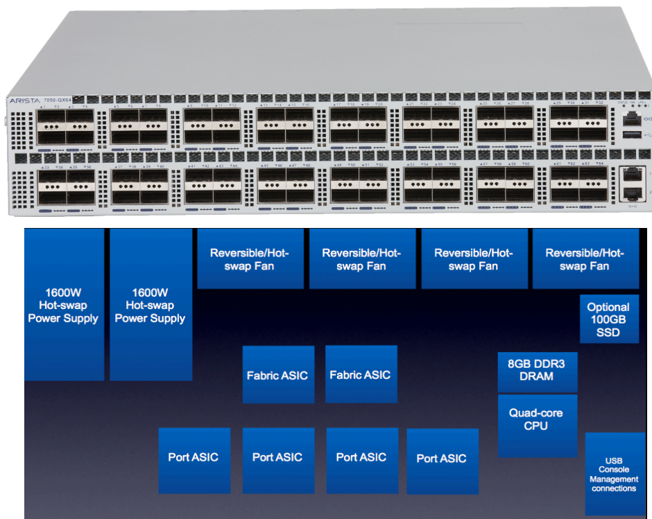
Figure 4: Arista 7250QX-64 (above: Physical Image, below: Logical device layout)
